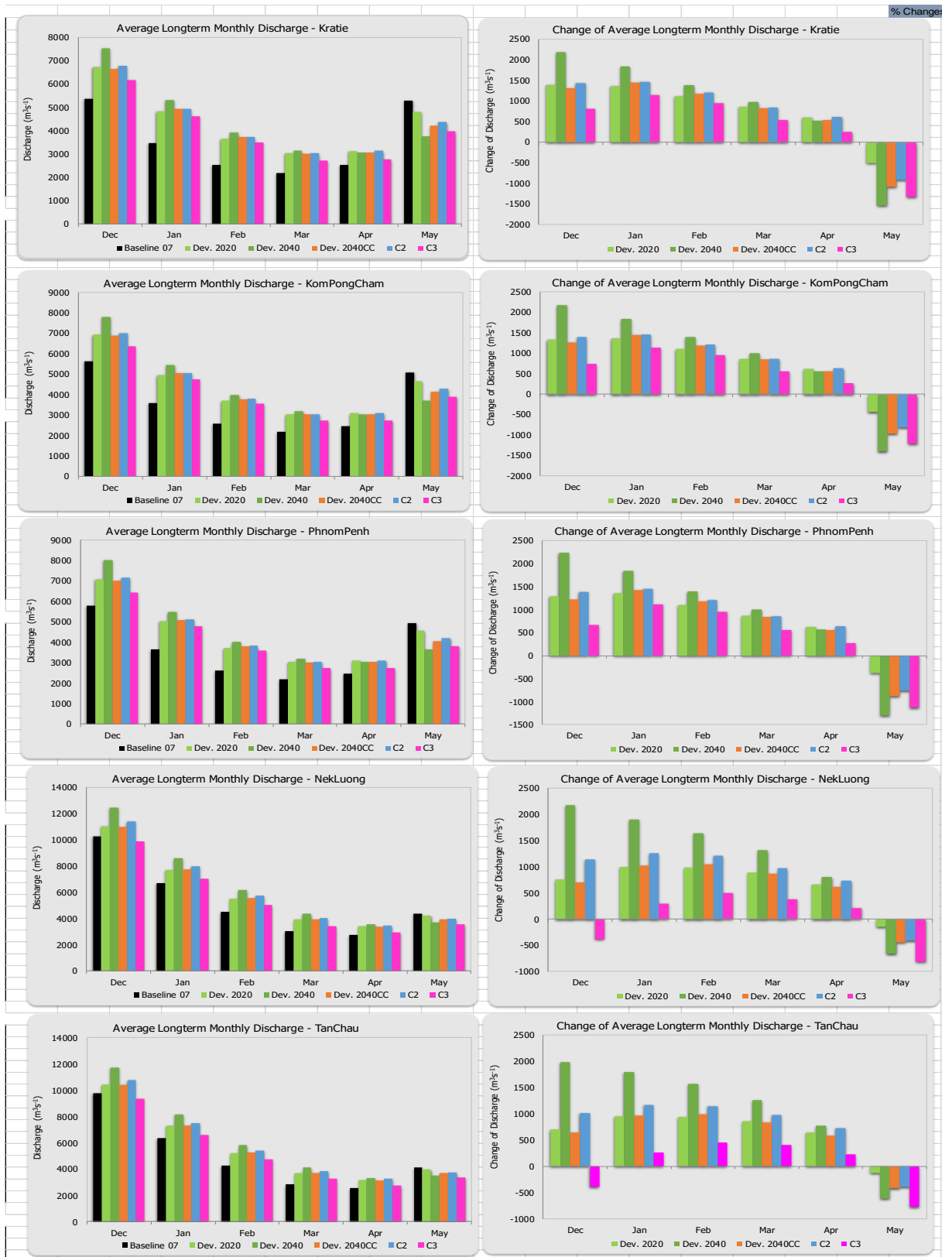
Figure 3 Dry Season Average Monthly Flow Key Station Kratie -Tan Chau
